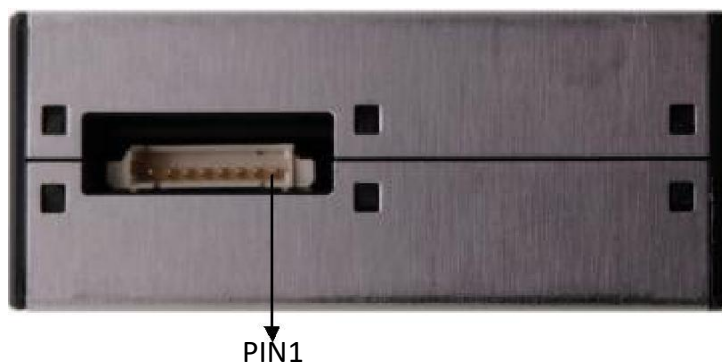
Figure 2 Connector Definition
